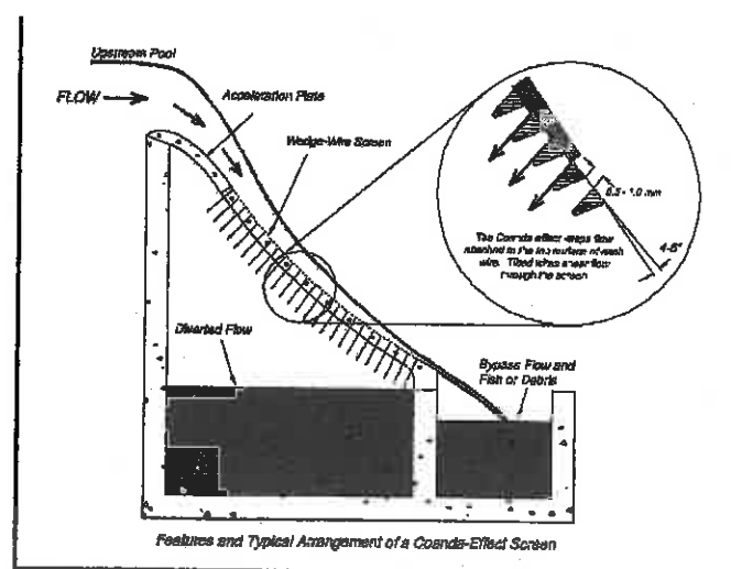
Figure 5. Operating principles of a Coanda stormwater filtration screen. (Image taken from Wahl, Tony L., 2003, Design Guidance for Coanda-Effect Screens. U.S. Dept. of the Interior, Bureau of Reclamation, Research Report R-03-03. July 2003. [online paper]).
