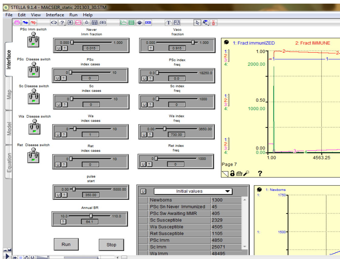
Figure 14: MACSEIR Interface
