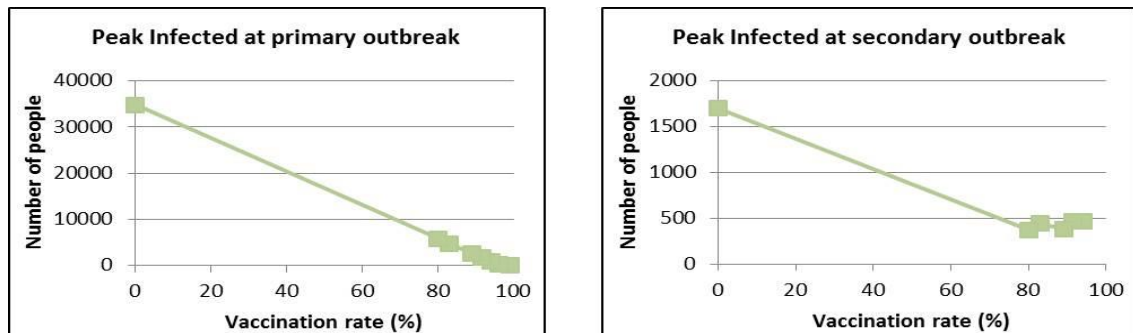
Figure 19: Peak infected for static vaccination rate
