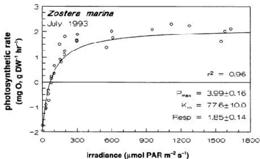
Figure 2.1 Exemplary photosynthesis-irradiance curve of a seagrass (specifically intertidal Zostera marina from the Zandreek, SW Netherlands). P_{\max} , K_m and \text{Resp} are the maximum photosynthetic rate, saturating irradiance, and respiration terms respectively. Adapted from Vermaat (1997).
