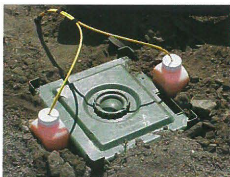
Figure 1. FIXOR counter-force or "earmuff" attack configuration.
