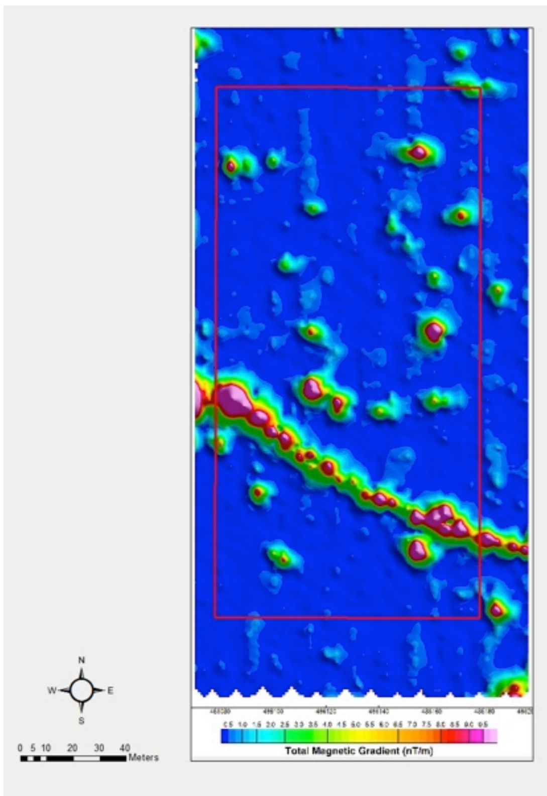
Figure C-3. Processed total field magnetometer data from AUV-towed Marine Magnetics Explorer magnetic sensor in the in-shore field survey.
