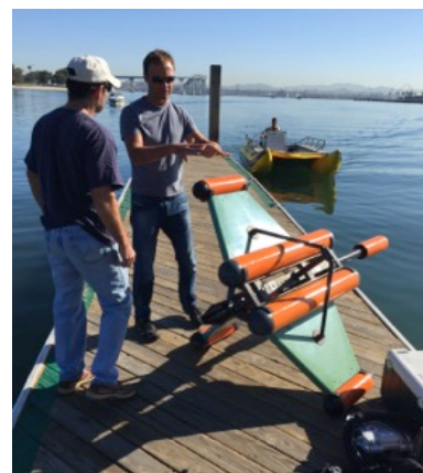
Figure 3. SeaQuest operator conducting pre-mission checks.
