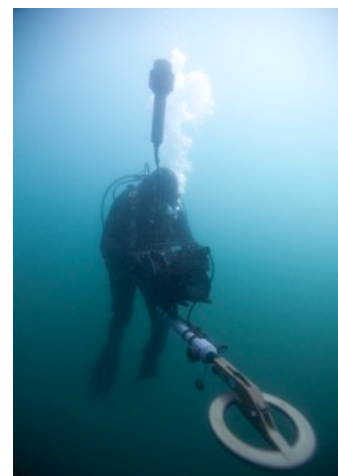
Figure 5. Scuba diver with Shark Marine Underwater Navigation System with metal detector attachment.
