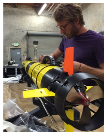
Figure 1. Iver3 AUV operator conducting pre-mission checks.
