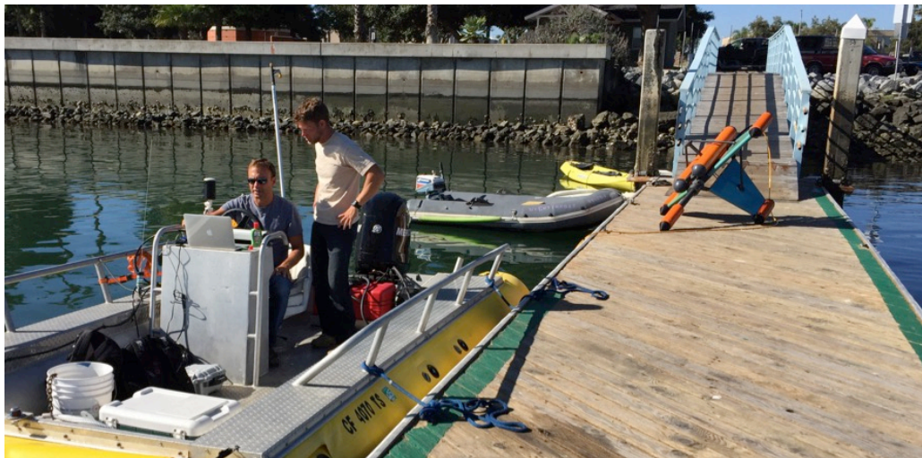
Figure 12. Marine Magnetism SeaQuest magnetometer on the pier.
