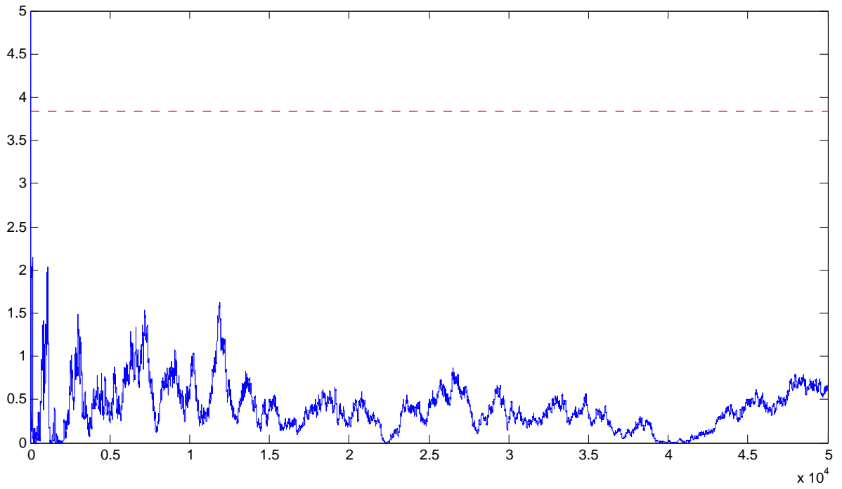
Figure 11: Chi Square Test Results - Fair Coin, 50000 Trials
